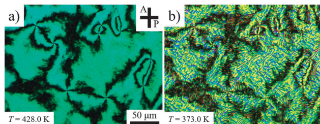
Fig. 6 POM textures in the SE7511 cell of d = 3.9 \mu\text{m} (a) at T = 428.0 \text{ K} (N phase) and (b) 373.0 \text{ K} ( N_{\text{TB}} phase).
