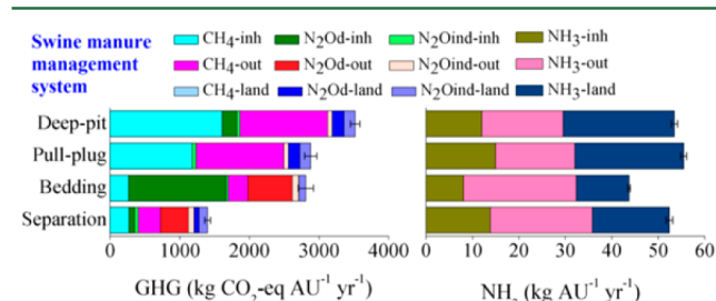
Figure 3. GHG and NH 3 emissions of baseline scenarios for deep-pit, pull-plug, bedding and separation systems as defined in Figure 1 (see Tab SummBaseEmi in Data set S1 for numeric data). N 2 O d = direct N 2 O emission; N 2 O i d = indirect N 2 O emission; in = in-house; out = outdoor; land = land application; AU = animal unit (1 AU = 500 kg).
