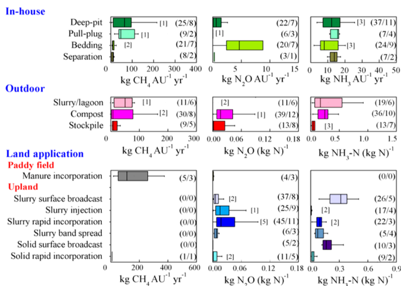
Figure 2. Box and whisker plots of the CH 4 , N 2 O and NH 3 emission factors for the various manure management practices in three phases (in-house, outdoor and land application) (see SI Table S3–S5 for numeric data). The vertical lines of the boxplots represent the median, upper and lower quartiles. The whiskers show values that extend to 1.5 orders of box length. The numbers in the square brackets represent the number of outliers (>1.5 orders of box length). Values in parentheses represent the number of observations on which the statistics were based and the number of studies from which the observations originated.
