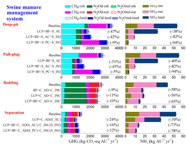
Figure 5. GHG and \text{NH}_3 emissions of baseline scenarios and recommended mitigation scenarios for deep-pit, pull-plug, bedding and separation systems, with baseline scenarios defined in Figure 1; the numbers in parentheses indicate the mitigation efficiency (see DeepPitSystem tab, PullPlugSystem tab, BeddingSystem tab and SeparationSystem tab in Data set S1 for numeric data). \text{N}_2\text{Od} = direct \text{N}_2\text{O} emission; \text{N}_2\text{Oind} = indirect \text{N}_2\text{O} emission; in = in-house; out = outdoor; land = land application; LCP = low crude protein; BF = biofilter; S_AC = slurry acidification; S_PC = slurry plastic cover; S_INJ = slurry injection; C_AD = compost additive; C_INC = compost incorporation; AU = animal unit (1 AU = 500 kg).
